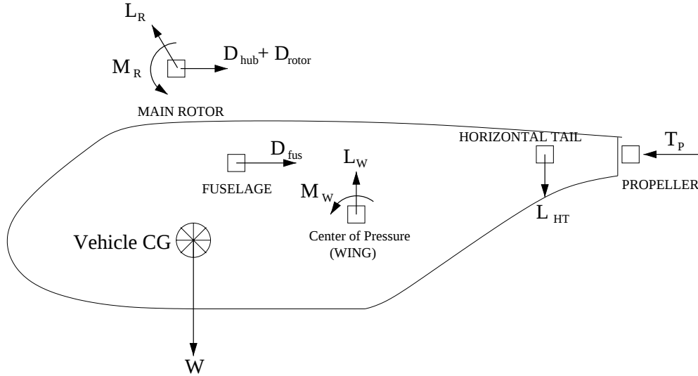
Figure 4.17: Vehicle trim in cruise (not to scale).
