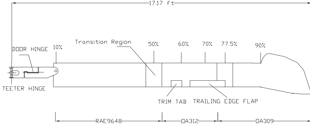
Figure 4.2: Blade and hub schematic (not to scale).
