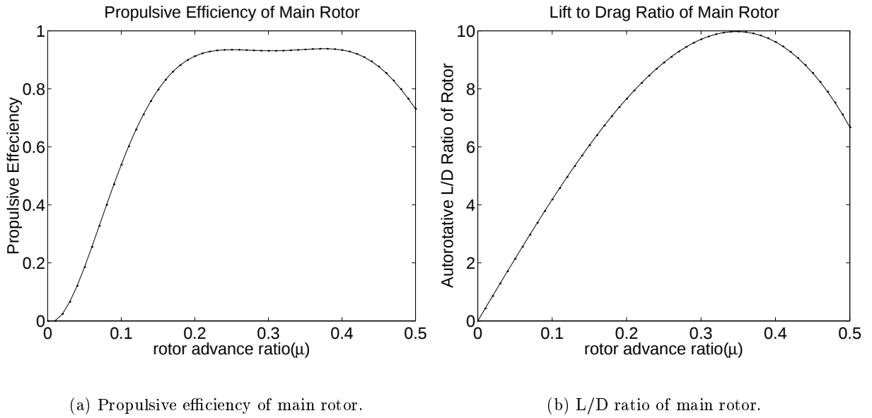
Figure 6.1: Effect of advance ratio on propulsive efficiency and lift/drag ratio of main rotor.
