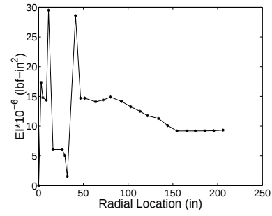
(b) Chordwise blade stiffness distribution.
