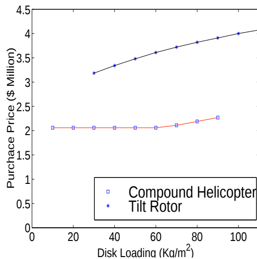
(b) Purchase price vs. disk loading.
