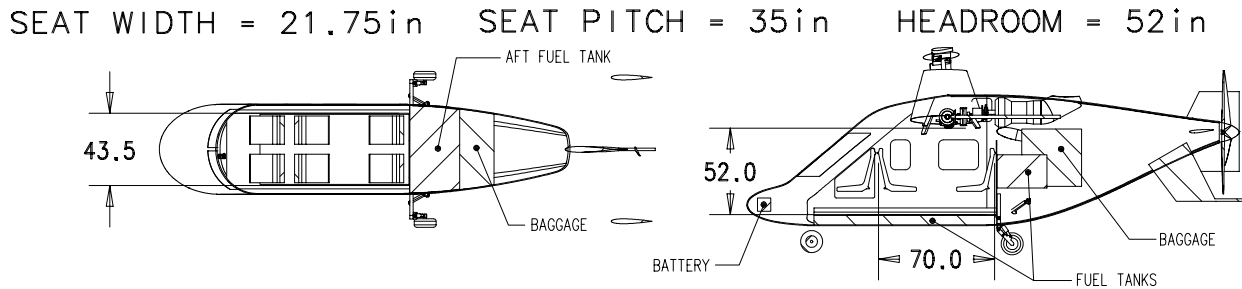
Figure 4.23: Cabin layout.
