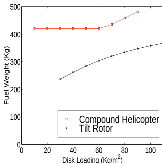
(b) Fuel weight vs. disk loading.
