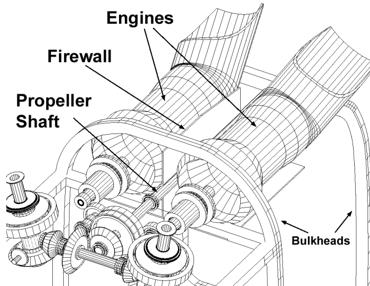
Figure 4.18: Engine installation.
