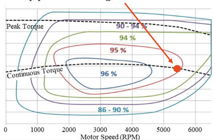
Efficiency Plot overlaid on Torque vs. RPM for EMRAX 188
