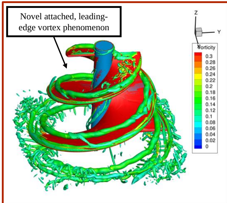
Visualization of vorticity on rotor with R_{\max} = 1.518\text{m}
