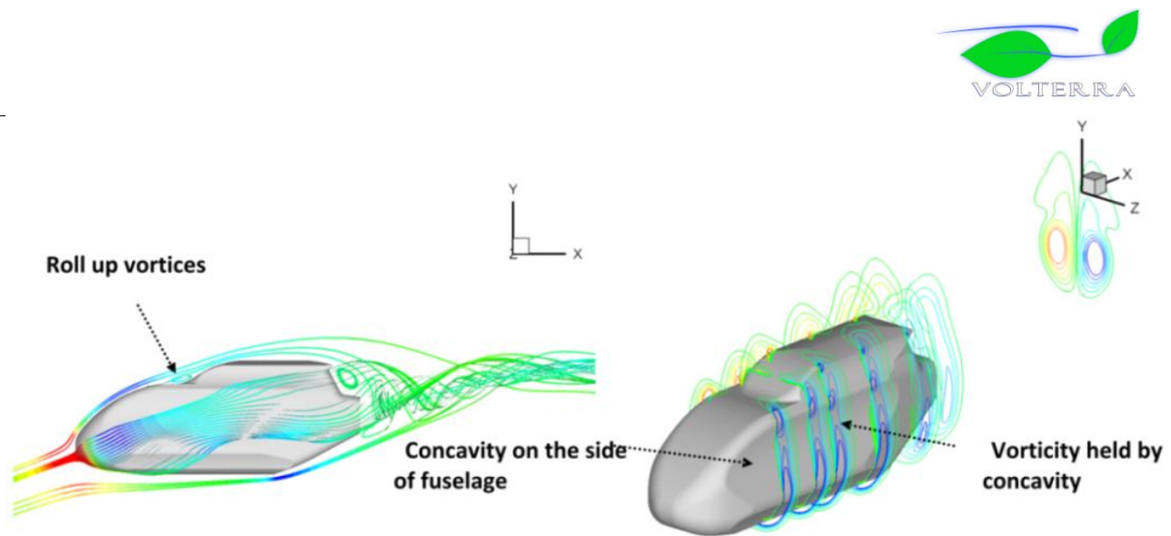
Figure 8.1: Flow over the modified fuselage of the EC-120 with concavity on the sides.
