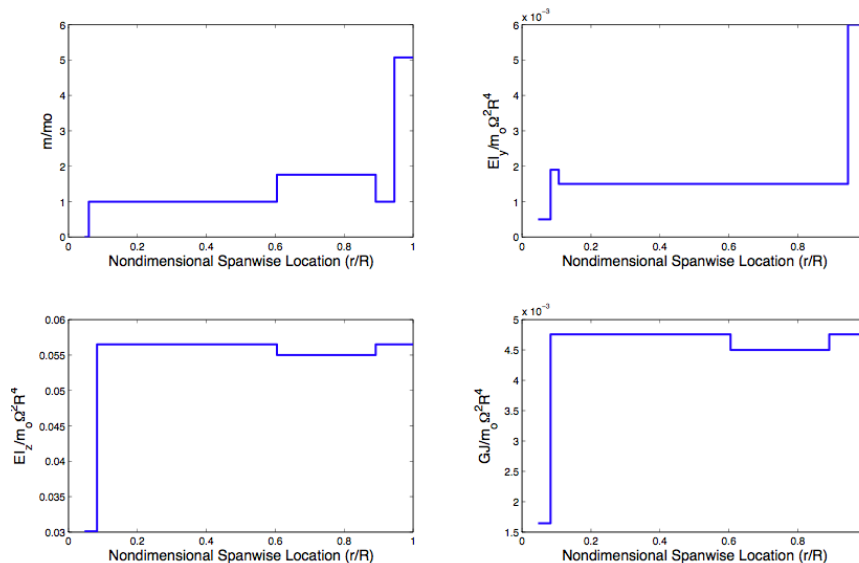
Figure 5.19: Blade mass and stiffness distribution.
