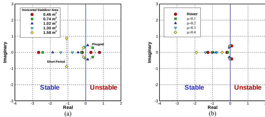
Figure 10.1: Longitudinal mode stability with (a) increases in horizontal stabilizer area ( \mu=0.3 ) (b) increases in forward flight speed (Area = 1.30 \text{ m}^2 )
