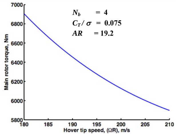
Figure 3.11: Variation of main rotor torque required with hover tip speeds.
