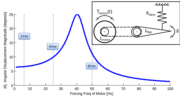
Figure 5.16: Frequency Response of Trailing Edge Flap Actuator
