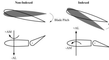
Figure 5.5: Blade indexing.
