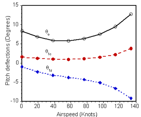
Figure 5.7: Pitch deflection angles for conventional swashplate rotor
