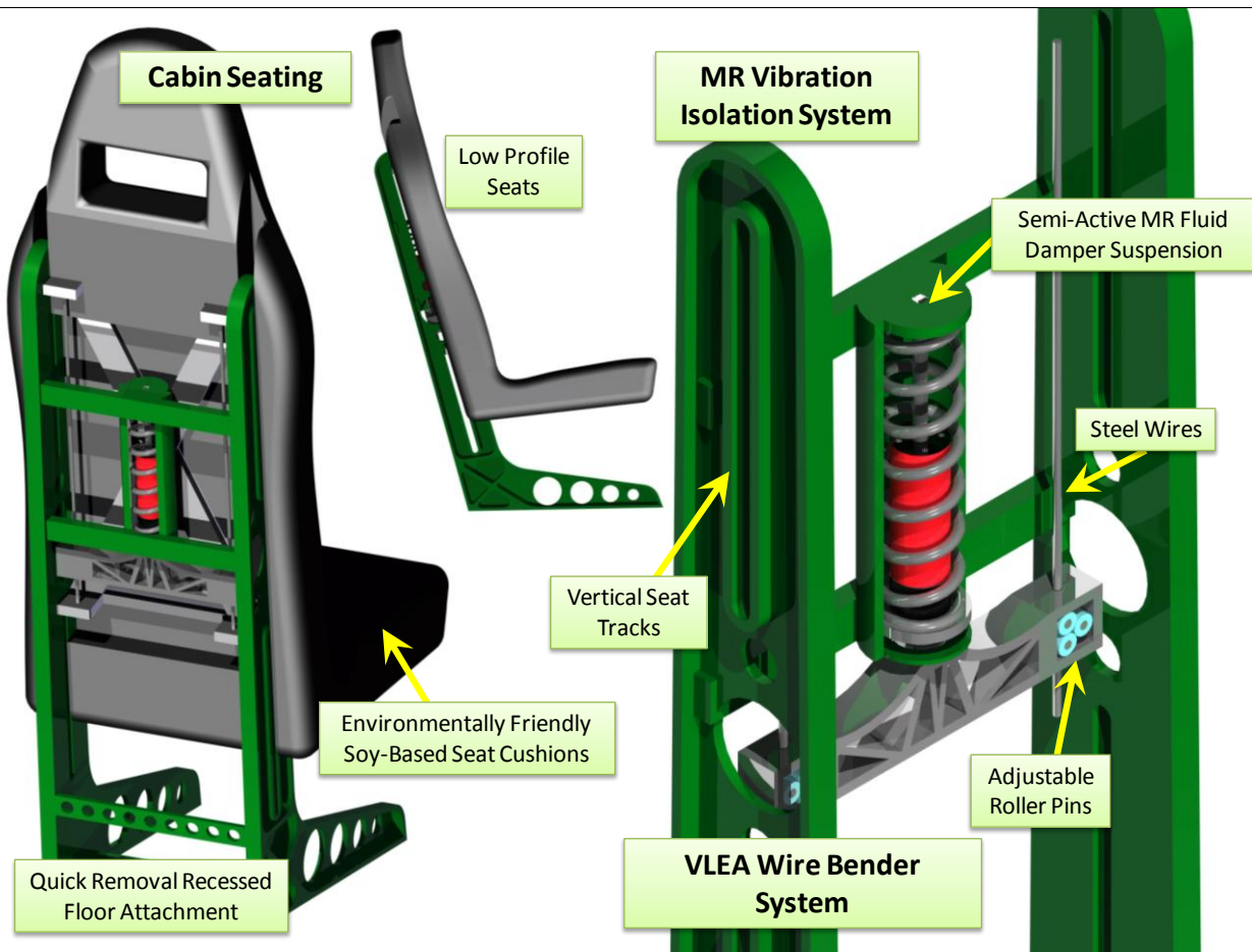
Figure 12.2: Cabin occupant seat design showing VLEA wire bender stroking system and vibration isolation system.
