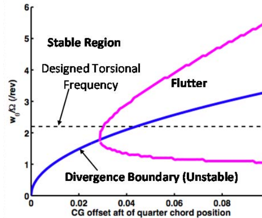
Figure 5.21: Stability Boundary for Pitch Flap Divergence and Flutter
