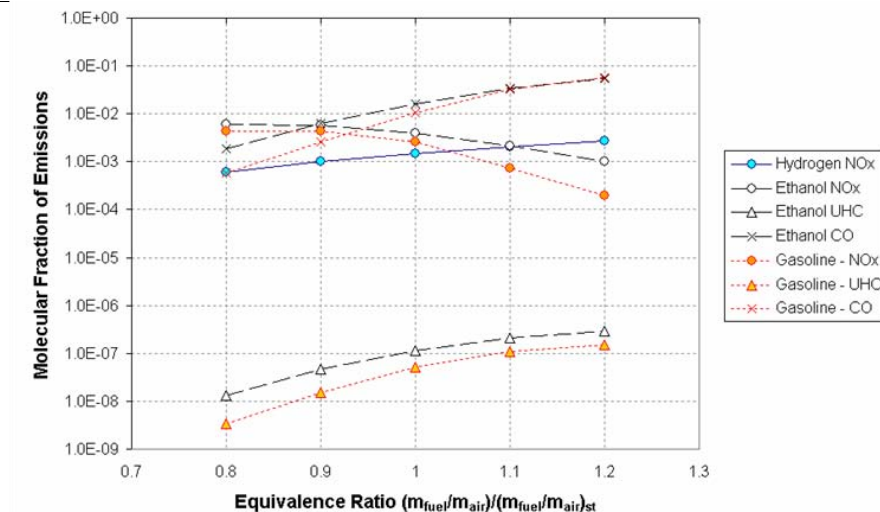
Figure 4.2: Emissions by equivalence ratio
