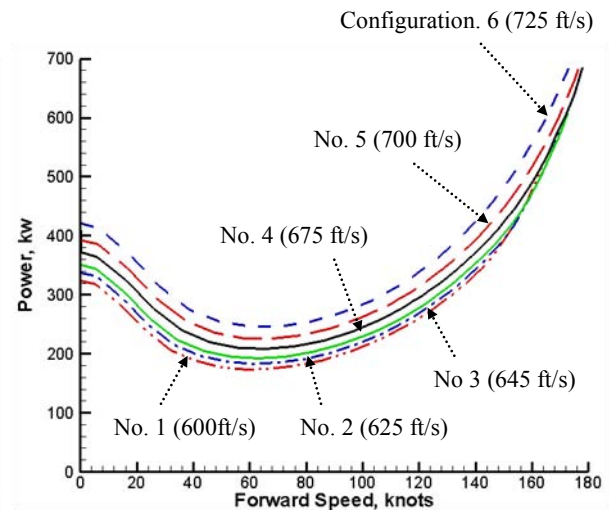
Figure 3.13: Variation of power required with forward speeds for 6 helicopter configurations designed at different tip speeds.
