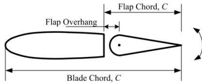
Figure 5.4: Cross-sectional parameters of a trailing-edge flap.
