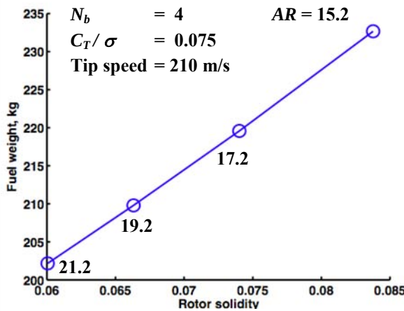
Figure 3.8: Variation of fuel required with rotor solidity.
