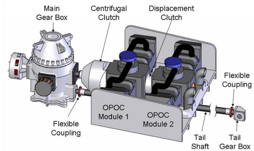
Figure 4.5: Transmission diagram
