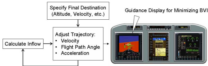
Figure 9.8: Flight path management system overview.
