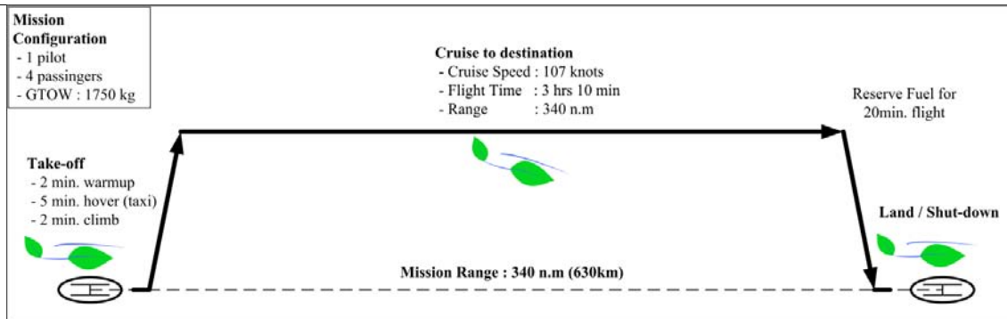
Figure 16.3 Standard mission profile
