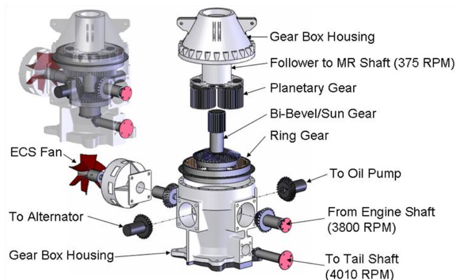
Figure 4.6: Main Gear Box.
