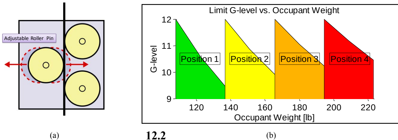
Figure 12.1: (a) Adjustable Roller Pins for Wire Bender VLEA, (b) Schematic of the limit load adjustment settings
