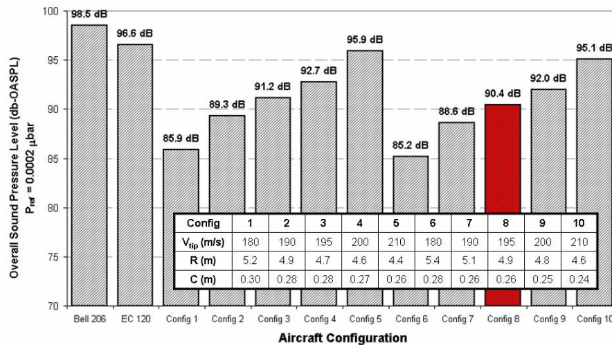
Figure 9.3: Sound pressure level of various 4-bladed rotor designs considered. 30° below tip-path plane at 10 rotor radii
