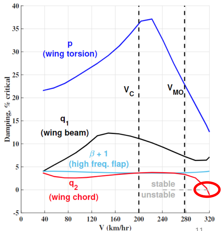
Clear of whirl flutter and air resonance
