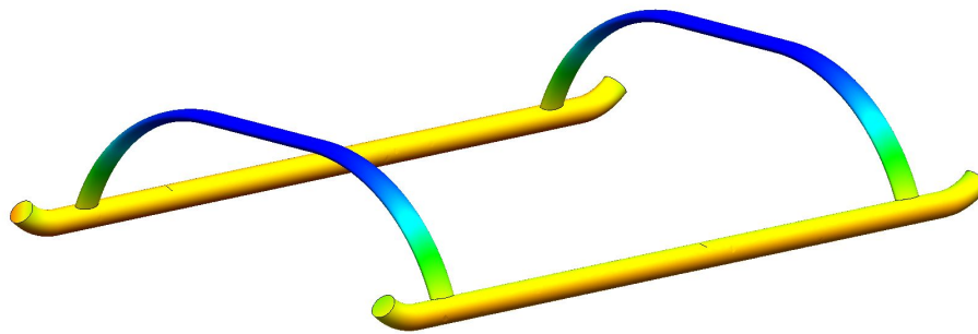
Deformation of landing gear
