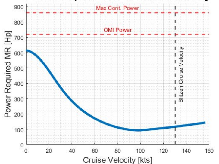
Power Required MR vs Cruise Velocity
