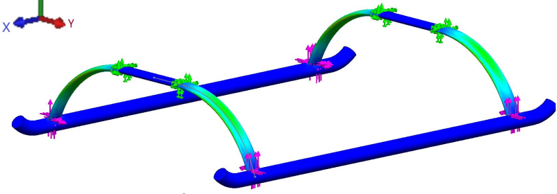
Stress on landing gear
