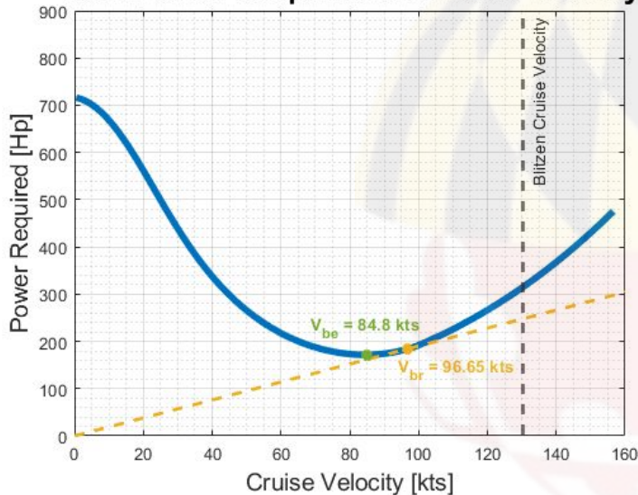
Power Required RotorProp vs Cruise Velocity
