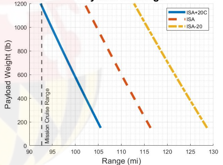
Payload vs Range
