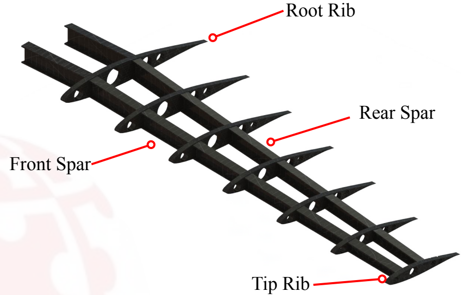
Wing structure with 7 ribs on each wing
