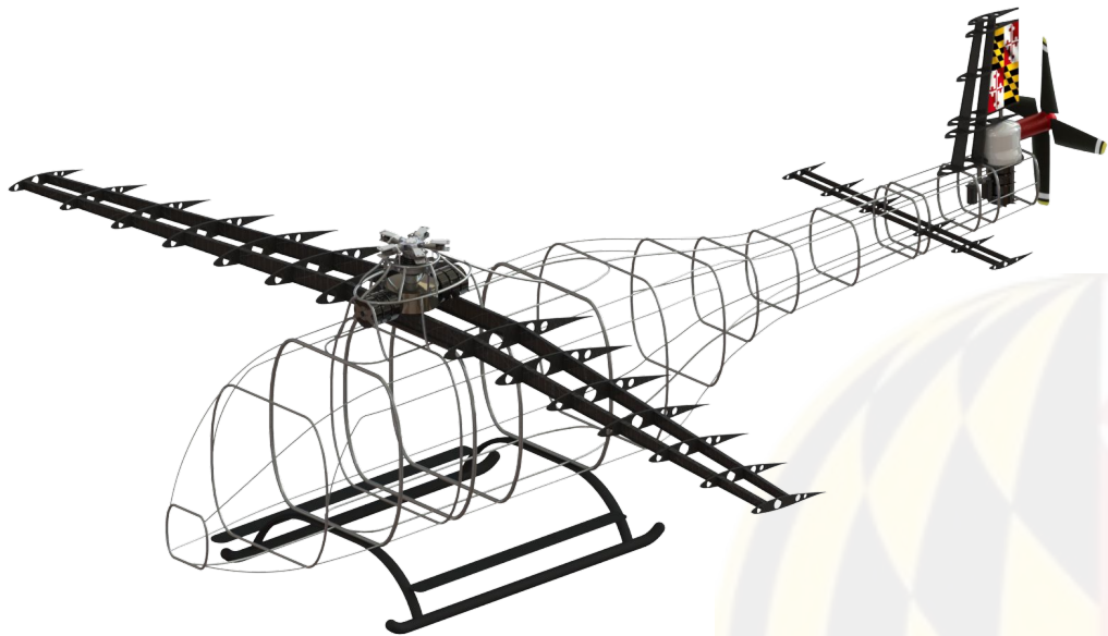
Fuselage airframe structure consisting of 10 primary I-beam bulkheads and 7 tail bulkheads
