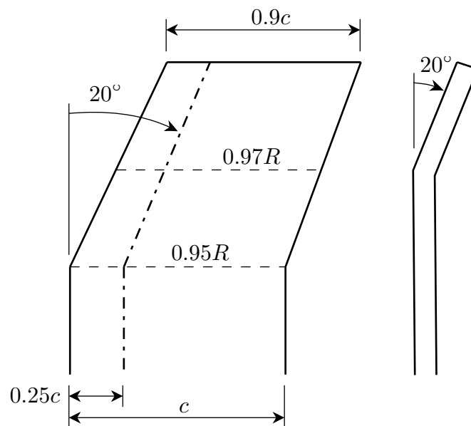
Figure 4.20: Tip geometry
