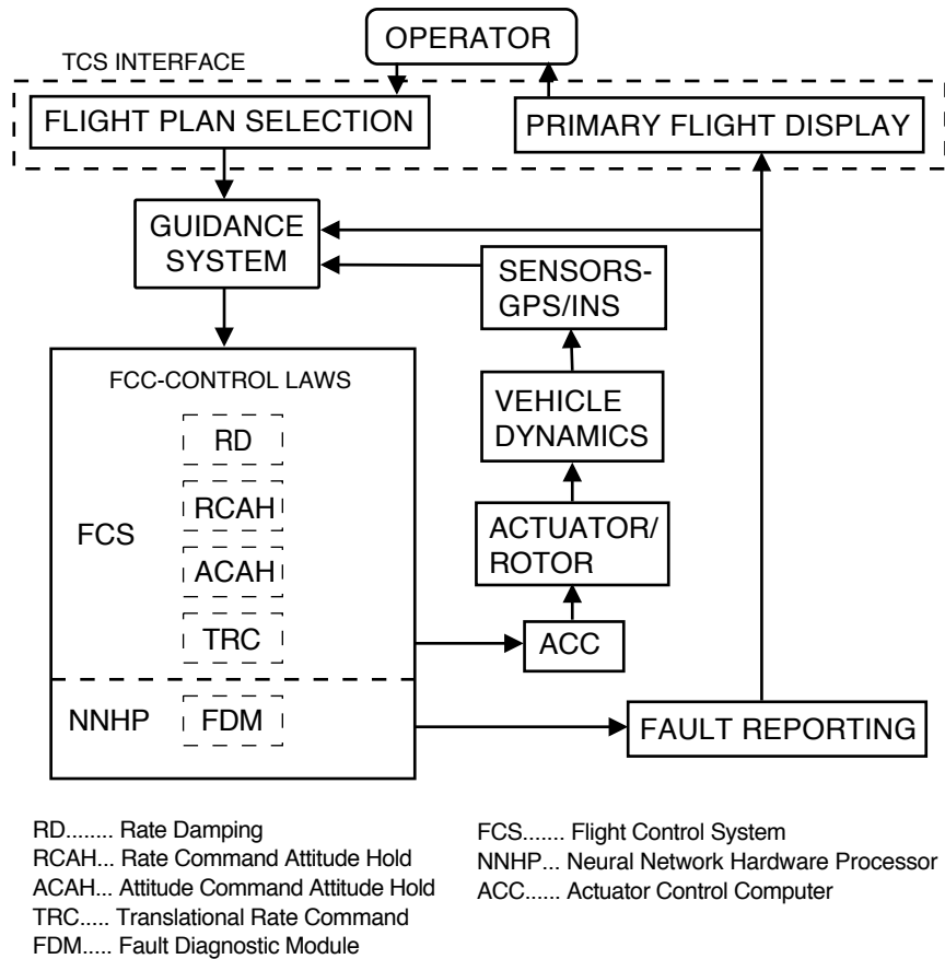
Figure 9.1: Architecture of automatic flight control system
