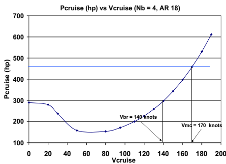
Figure 11.4: Required Power versus Speed
