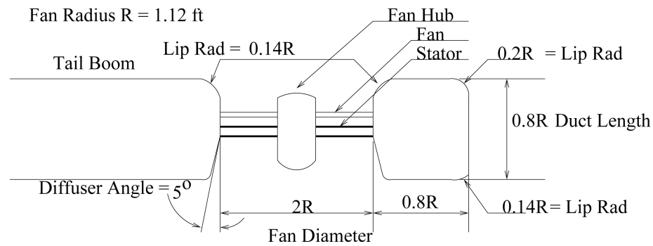
Figure 5.1: Sketch of Duct/Shroud Structure
