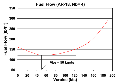
Figure 11.5: Fuel Flow versus Speed
