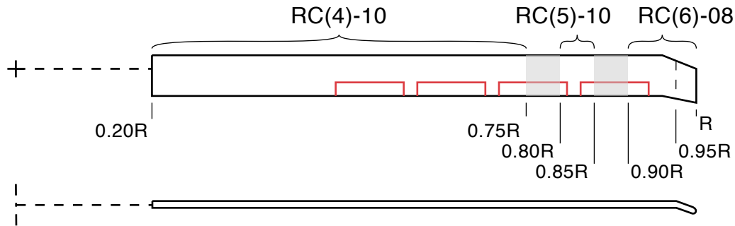
Figure 4.19: Airfoil distribution
