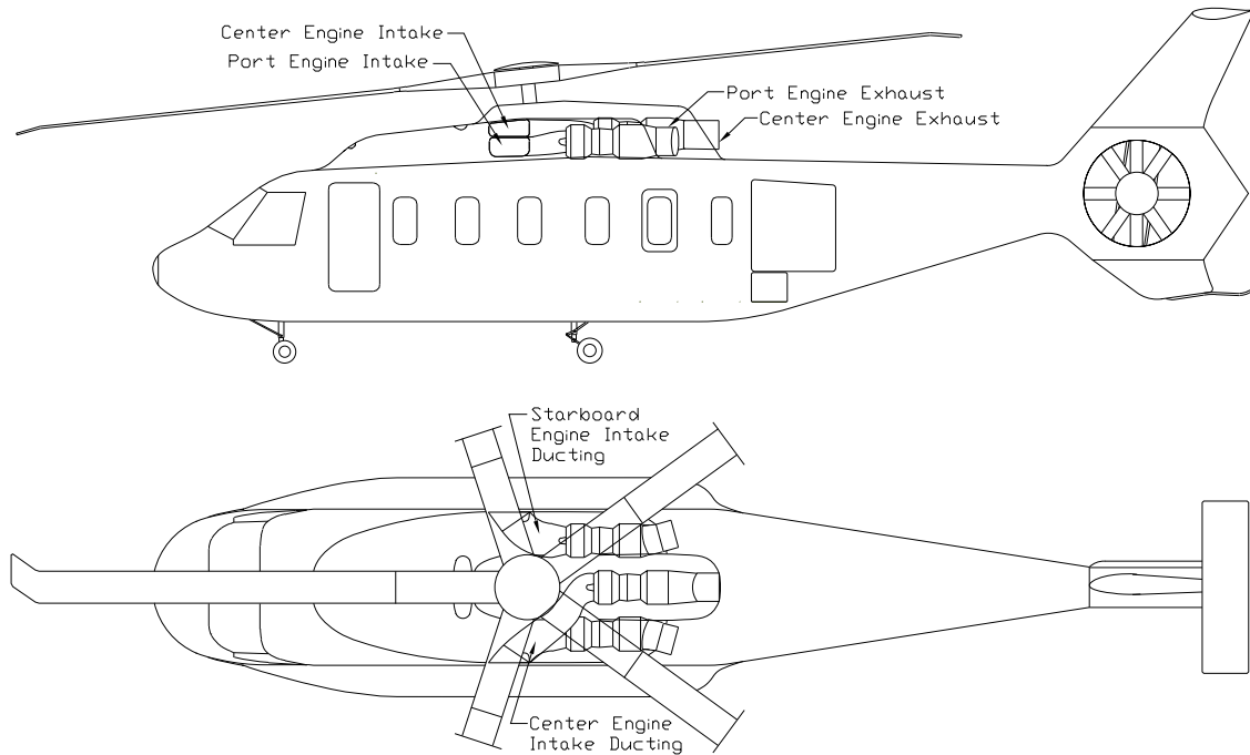
Figure 8.4: Engine installation
