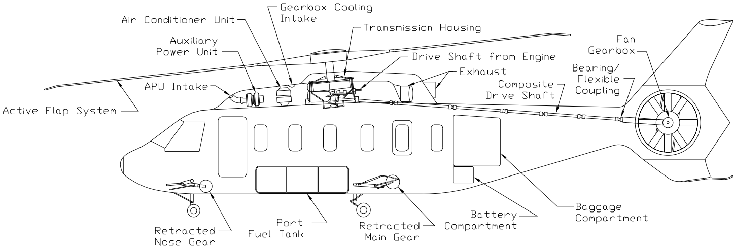
Figure 5.3: Aircraft Systems
