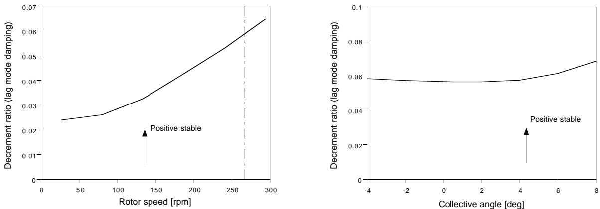
Figure 10.17: Ground resonance: lag mode damping with rotor speed Figure 10.18: Ground resonance: lag mode damping with collective angle
