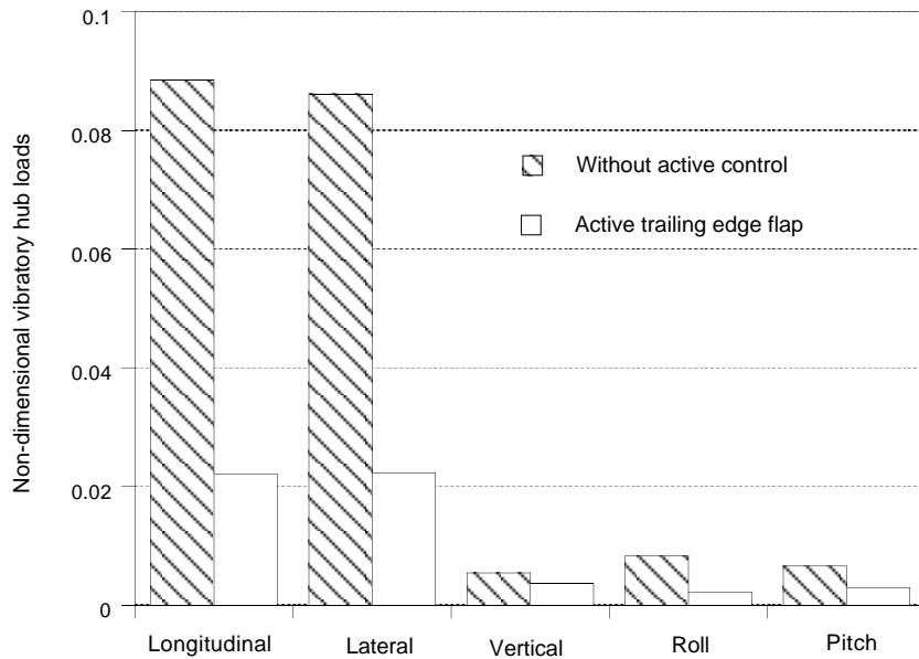
Figure 10.14: 5/rev Vibratory hub loads in cruise
